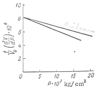
Fig. 7. Compressibility of strontium as a function of pressure. The upper curve was obtained by Bridgman.
