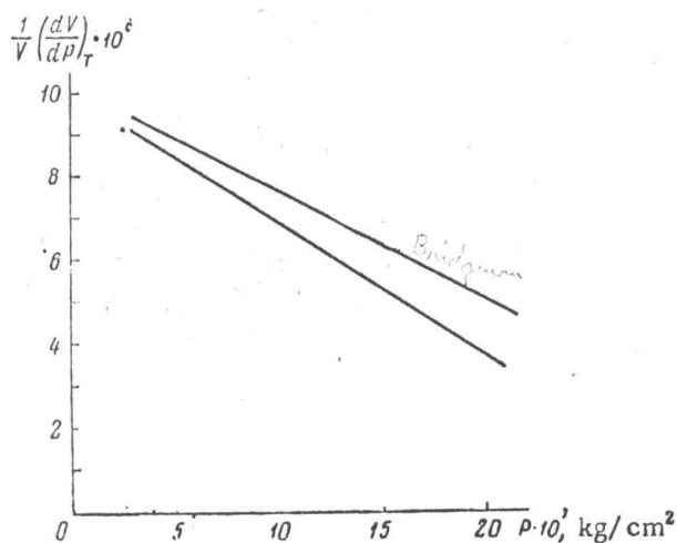
Fig. 8. Compressibility of barium as a function of pressure. The upper curve was obtained by Bridgman.
